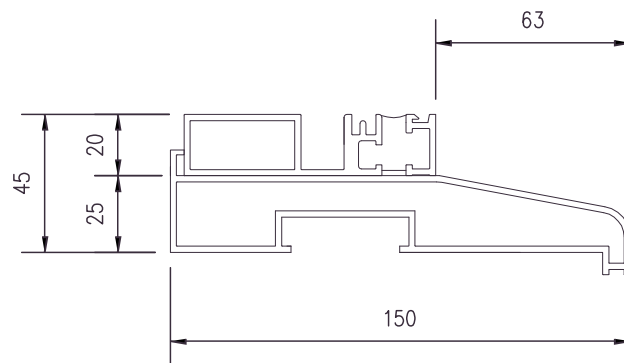
Low threshold with 150mm cill
