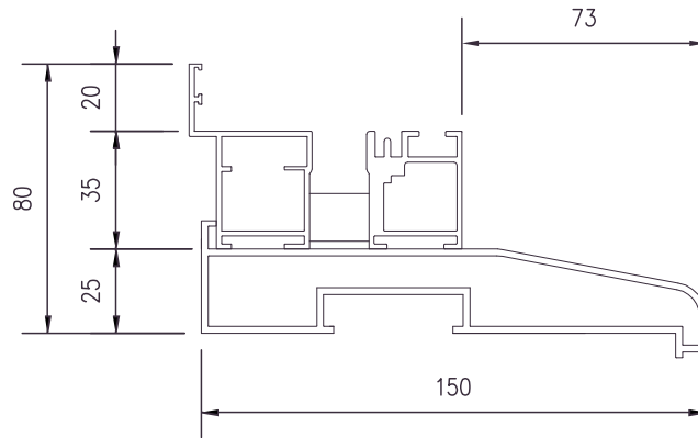
Standard threshold with 150mm cill
