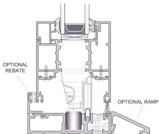
Low threshold detail
