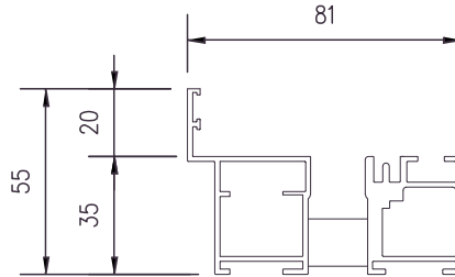
Standard threshold - no cill
