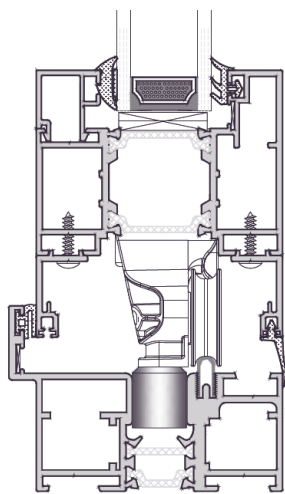
Standard threshold detail
