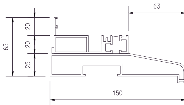
Low threshold with rebate and 150mm cill
