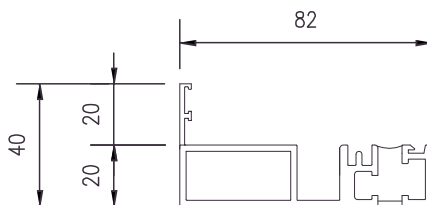
Low threshold with rebate - no cill
