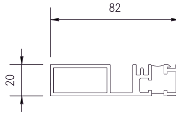
Low threshold - no cill
