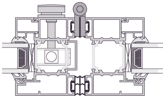
Intermediate detail integrated lock
