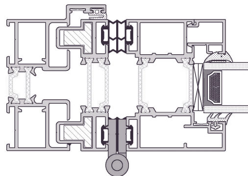
Outer frame detail with adjustable jambs
